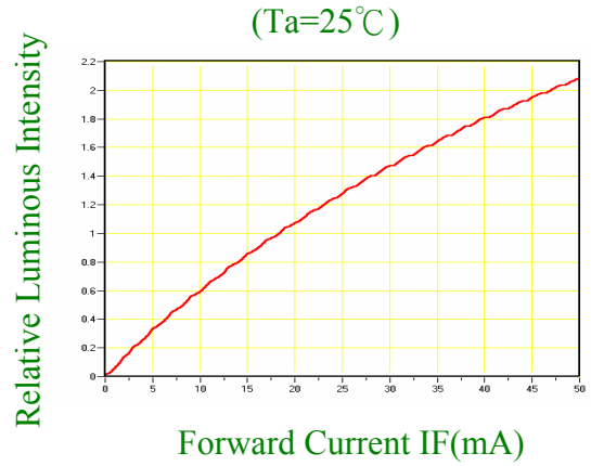
Relative Luminous Intensity-IF
