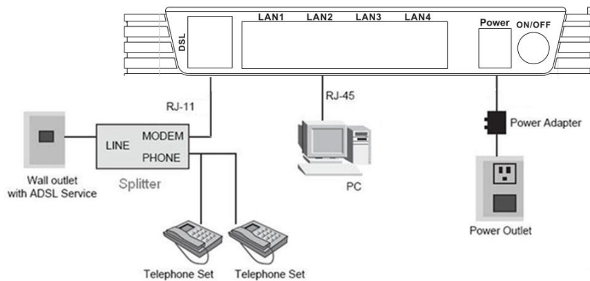
Figure 1 –Connection diagram (Without connecting telephone sets before the splitter)
