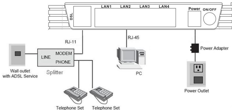
Figure 2 - Connection diagram (Connecting a telephone set before the splitter)
