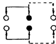
SCHEMATIC (NON-SHORTING)
