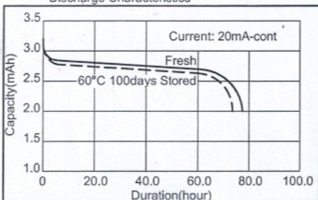
Discharge Characteristics
