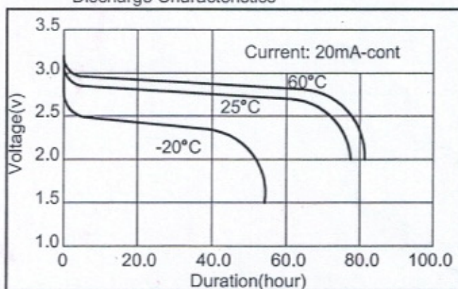
Discharge Characteristics
