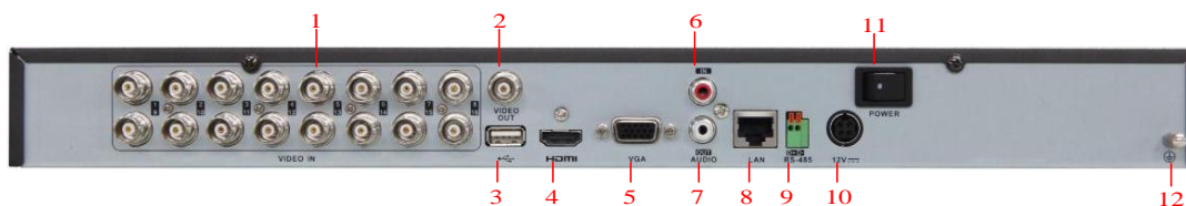
Figure 1.6 Rear Panel of 16CH DVR
