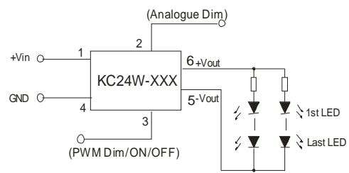
(Figure 2) Parallel-series Application
